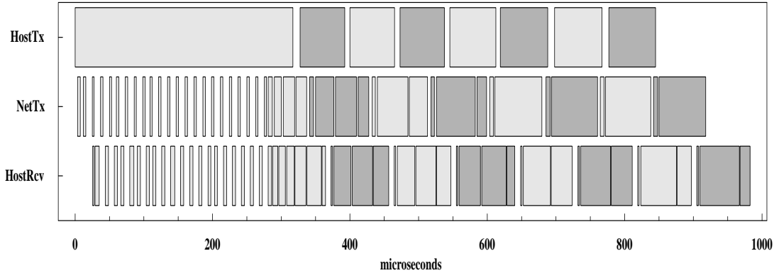
Figure 3: Adaptive message pipelining reverts to larger transfer sizes for a stream of 8K payloads. The fixed-size transfer at the start of each packet on NetTx and HostRcv is the control message data, which is always handled as a separate transfer. Control messages do not appear on HostTx because they are sent using programmed I/O rather than DMA on this platform (300 MHz Pentium-II/440LX).
