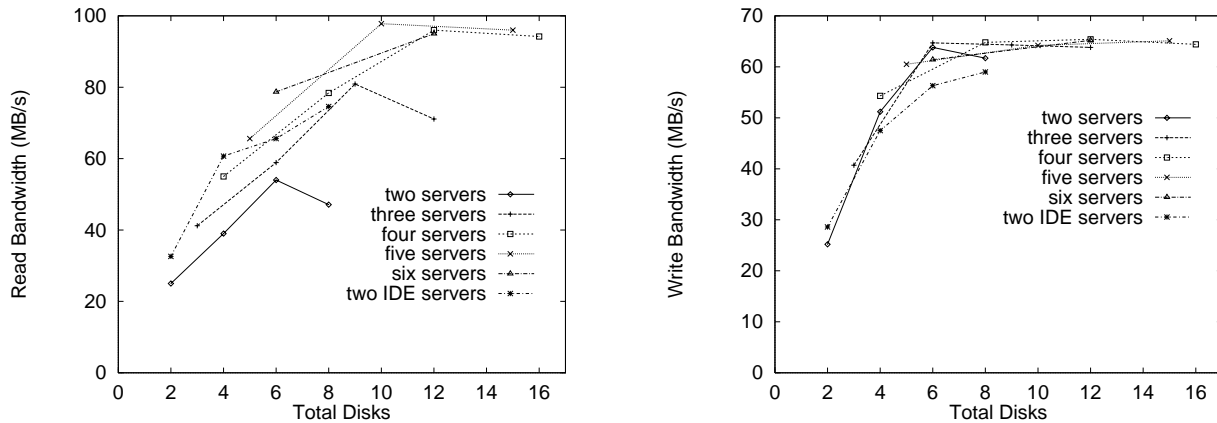
Figure 4: Single-client sequential disk read and write bandwidths with Slice/Trapeze.
