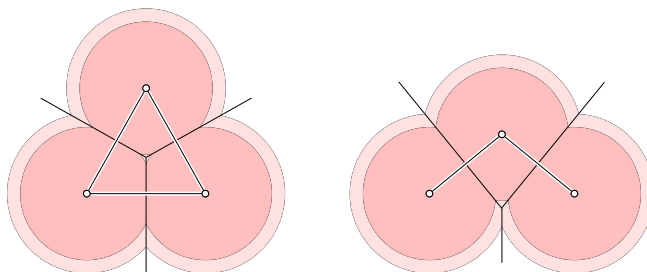
Figure III.18: Left: three points spanning an acute triangle. In the alpha complex evolution, the three edges appear first before the triangle enters as a critical simplex. Right: three points spanning an obtuse triangle. Two edges appear first and the triangle enters together with the third edge.
