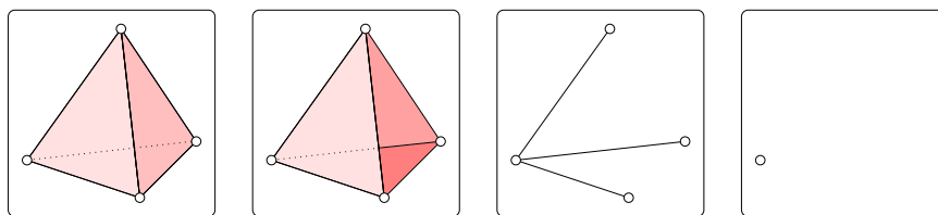
Figure III.17: From left to right: a tetrahedron, the three triangles left after a (2, 3) -collapse, the three edges left after three (1, 2) -collapses, the vertex left after three (0, 1) -collapses.
