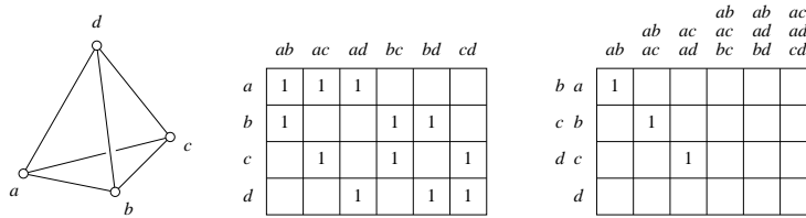
Figure IV.10: From left to right: the edge skeleton of the tetrahedron, its first boundary matrix, the reduced boundary matrix with rank \mathbf{B}_0 = 3 non-zero rows and rank \mathbf{Z}_1 = 3 zero columns.
