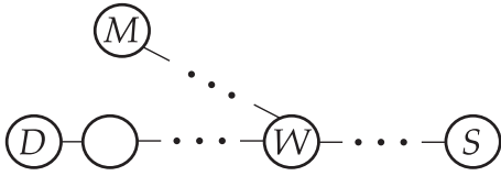
Figure 1: Prefix hijacking
