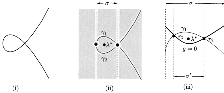
Fig. 8. (i) Roots of p ; (ii) cylindrical algebraic decomposition of p ; (iii) curves g = 0 and \gamma_1 .
