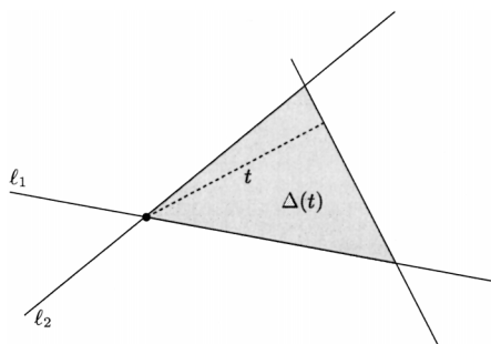
Fig. 7. An extremal-placement query.
