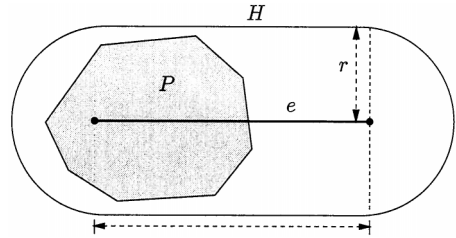
Fig. 4. The segment-center problem.
