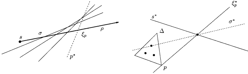
Fig. 6. A ray-shooting query.
