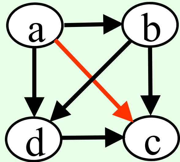
Slater ranking
