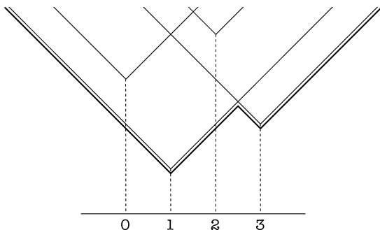
Figure 1. An illustration of the lower envelope of four cones in the case of one-dimensional labels (e.g., stereo disparity or image restoration). Each cone is rooted at location (f_p, h(f_p)) . The darker line indicates the lower envelope.
